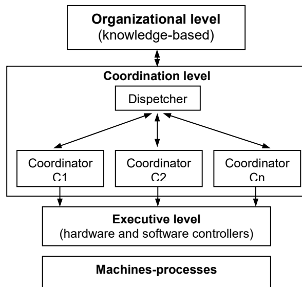
Figure 1. The generally accepted structure of intelligent control
